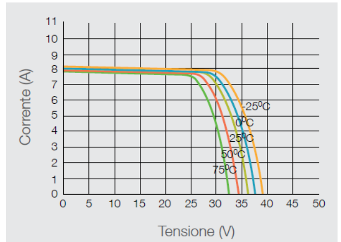
Fig. 1: IV curve at different irradiances
